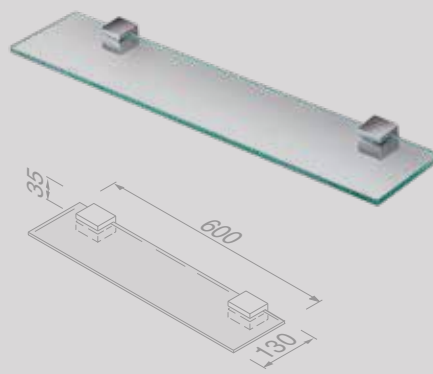
Planchet 60 cm Bathroom shelf 60 cm 917545-02
