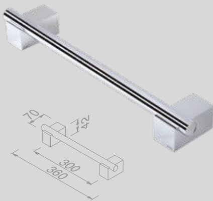
Badgreep 30 cm Grab rail 30 cm 917506-02
