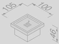
Zeephouder Soap holder 913503-02
